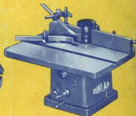
99 PT 02317—DUNLAP Shaper. Table, 15 1/8 x 10 1/2 in. Page 13
